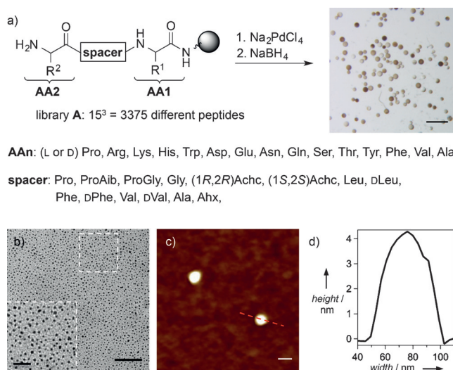
Figure 1. a) General structure of library A and combinatorial assay for PdNPs (scale bar 50 \mu m). [15] b) TEM image of PdNPs generated in the presence of 1 (scale bars 50 nm and 15 nm in expansion). c) AFM tapping mode micrograph of PdNP@ 1 (scale bar 50 nm). d) Cross-section along the broken red line of the AFM micrograph in (c).
